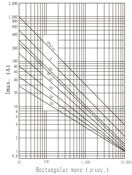
PULSE LIFETIME RATINGS- 14mm 14N180M~14N680K
