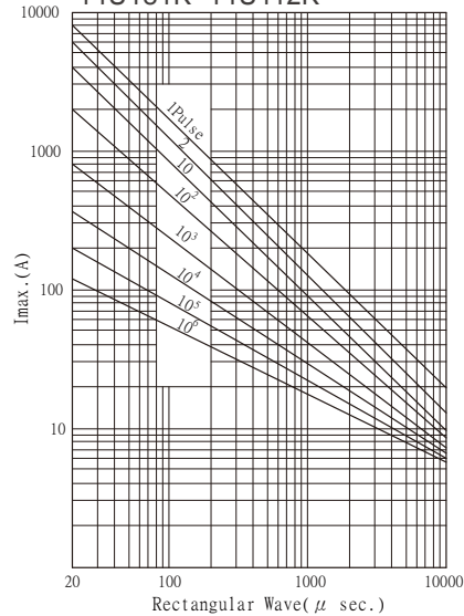
PULSE LIFETIME RATINGS- 14mm 14U181K~14U112K
